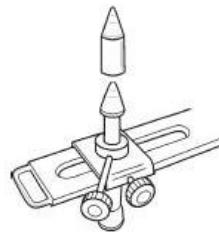
KIT SR – Wheel support
